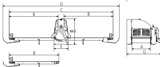
SB500-100/120
