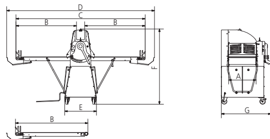
ST500-100/120
